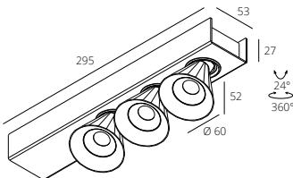
RSLC74131-3/3x7W
