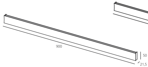
RWLB146/30W-90
