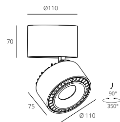
RSLC7560/28W
