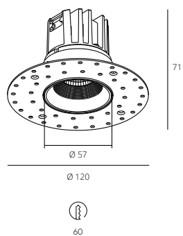
RSL74236/10W
