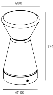
RTD3001/3W
