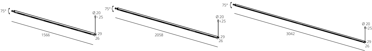
RHL77010/30W
