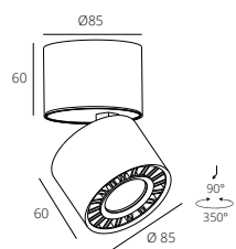
RSLC7529/12W
