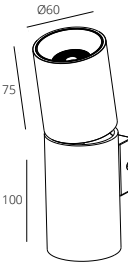
RWLB091/2x5W
