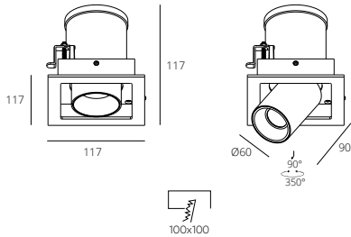
RGL7117-1/1x12W
